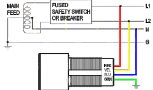
SINGLE PHASE, 3W + GND
