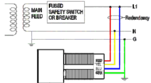
SINGLE PHASE, 2W + GND
