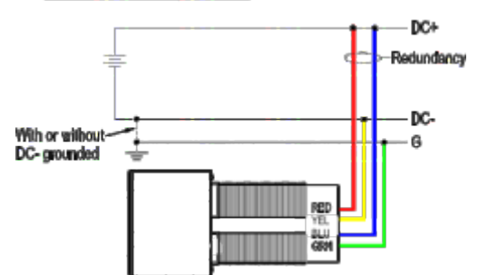
DC SINGLE SOURCE, 2W + GND
