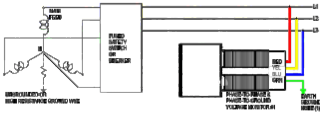
UNGROUNDED OR HIGH RESISTANCE GROUND WYE
