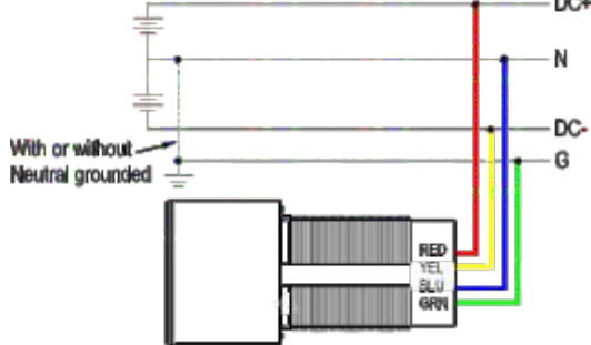
DC SPLIT SUPPLY, 3W + GND
